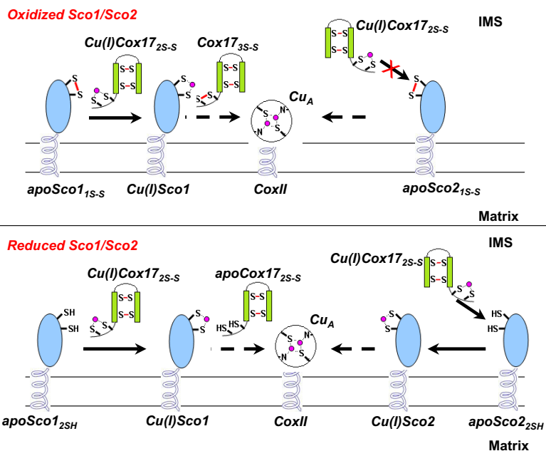
Fig. 4. Proposed mechanism of copper transfer from HCoX 17 25-5 to the subunit II of CcO, through the assistance of HSCO1 and HSCO2. This model implies that HSCO1, independently of the redox state of its Cys ligands in the IMS, may accept copper(I) from the mitochondrial chaperone Cu(I)HCoX 17 25-5 to form Cu(I)HSCO1 whereas HSCO2 can accept copper(I) from Cu(I)HCoX 17 25-5 only once its Cys ligands in the IMS are in a reduced state. HCoX 17 25-5 , produced by the redox HSCO1/HCoX 17 25-5 reaction, can be quickly reduced to HCoX 17 25-5 by GSH, thus the latter protein being recycled for the following metal transfer.
