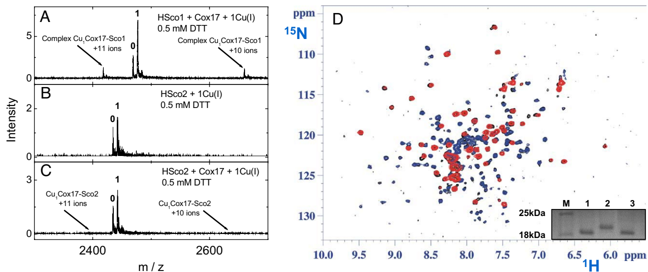
Fig. 3. Electro-spray ionization (ESI) MS analysis of Cu(I)HCo17 _{25-5} /HSco protein-protein complex formation in the presence of 0.5 mM DTT (Left) and NMR data on Cu(I)HCo17 _{25-5} /HSco2 _{15-5} mixture in the absence of reducing agents (Right). (A) Mixture of HSco1 (3 \mu\text{M} ), HCo17 _{25-5} (2 \mu\text{M} ), and Cu(I)DTT (2 \mu\text{M} ). (B) Mixture of HSco2 (3 \mu\text{M} ) and Cu(I)DTT (2 \mu\text{M} ). (C) Mixture of HSco2 (3 \mu\text{M} ), HCo17 _{25-5} (2 \mu\text{M} ), and Cu(I)DTT (2 \mu\text{M} ). Conditions: 20 mM ammonium acetate, pH 7.5, 0.5 mM DTT. ESI MS spectra were recorded as described in Materials and Methods. Charge state +8 ions are presented for HSco1 and HSco2, and numbers on the peaks denote the metal stoichiometry of the complex. Peaks corresponding to +10 and +11 ions of HCo17 _{25-5} /Cu(I) _1 /HSco1 complexes (A) and positions of theoretical peaks for HCo17 _{25-5} /Cu(I) _1 /HSco2 complexes (C) are indicated with arrows. (D) ^1\text{H}-^{15}\text{N} HSQC spectrum of a 1:1 ^{15}\text{N} -labeled HSco2 _{25-5} / ^{15}\text{N} -labeled Cu(I)HCo17 _{25-5} mixture (in black) overlaid with ^1\text{H}-^{15}\text{N} HSQC spectra of ^{15}\text{N} -labeled HSco2 _{15-5} (in blue) and of ^{15}\text{N} -labeled Cu(I)HCo17 _{25-5} (in red). The NH resonances of the mixture and of the starting materials are well superimposed and no new NH resonances of Cu(I)HSco1 and apoHCo17 _{25-5} species are detected, indicating that no reaction occurs. (Inset) Nonreducing SDS/PAGE gel. Lane M, protein marker; lane 1, HSco2; lane 2, AMS-modified HSco2 _{5\text{SH}} ; lane 3, AMS-modified HSco2 _{15-5} .
