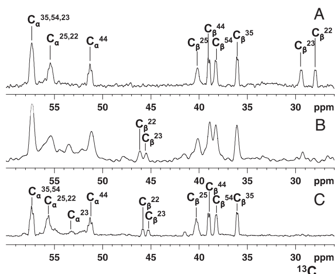
Fig. 2. Oxidation state of HCo17 cysteines monitored in the redox reaction between ( ^{13}\text{C},^2\text{H},^{15}\text{N} )Cys-selectively labeled Cu(I)HCo17 _{25-5} and ^{15}\text{N} -labeled HSco1 _{15-5} . Chemical shift changes of \text{C}^\alpha and \text{C}^\beta carbons of Cys residues of Cu(I)HCo17 _{25-5} were followed by 1D ^{13}\text{C} NMR spectra. (A) ( ^{13}\text{C},^2\text{H},^{15}\text{N} )Cys-selectively labeled Cu(I)HCo17 _{25-5} . (B) 1:1 ( ^{13}\text{C},^2\text{H},^{15}\text{N} )Cys-selectively labeled Cu(I)HCo17 _{25-5} / ^{15}\text{N} -labeled HSco1 _{15-5} mixture. (C) ( ^{13}\text{C},^2\text{H},^{15}\text{N} )Cys-selectively labeled HCo17 _{35-5} obtained by air oxidation. The assignment of the \text{C}^\alpha and \text{C}^\beta resonances of the Cys residues of both Cu(I)HCo17 _{25-5} and HCo17 _{35-5} forms is reported. \text{C}^\beta signals of the two Cys residues (C22 and C23) of Cu(I)HCo17 _{25-5} that are involved in the disulfide exchange reaction drastically reduce their intensity in the protein mixture (B) with the concomitant formation of the corresponding \text{C}^\beta signals with chemical shifts typical of HCo17 _{35-5} .
